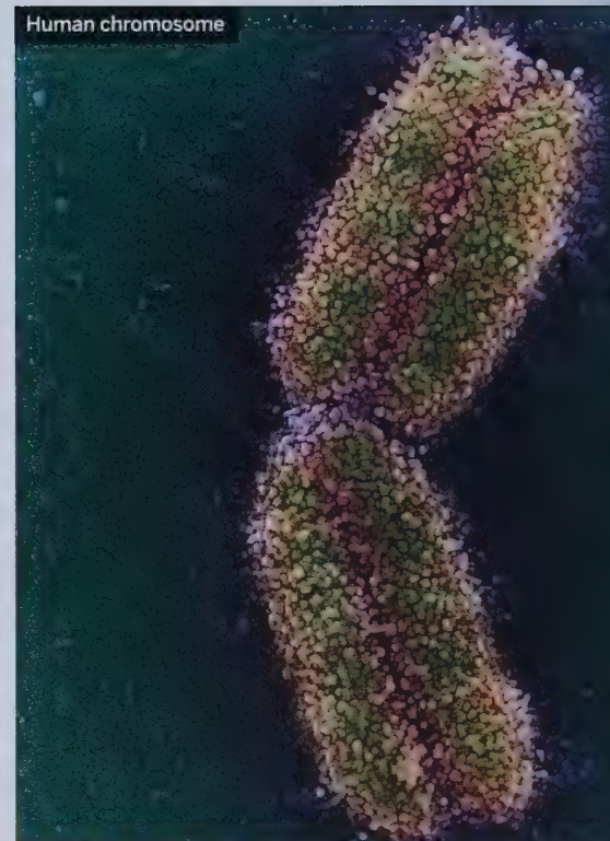
Human chromosome
